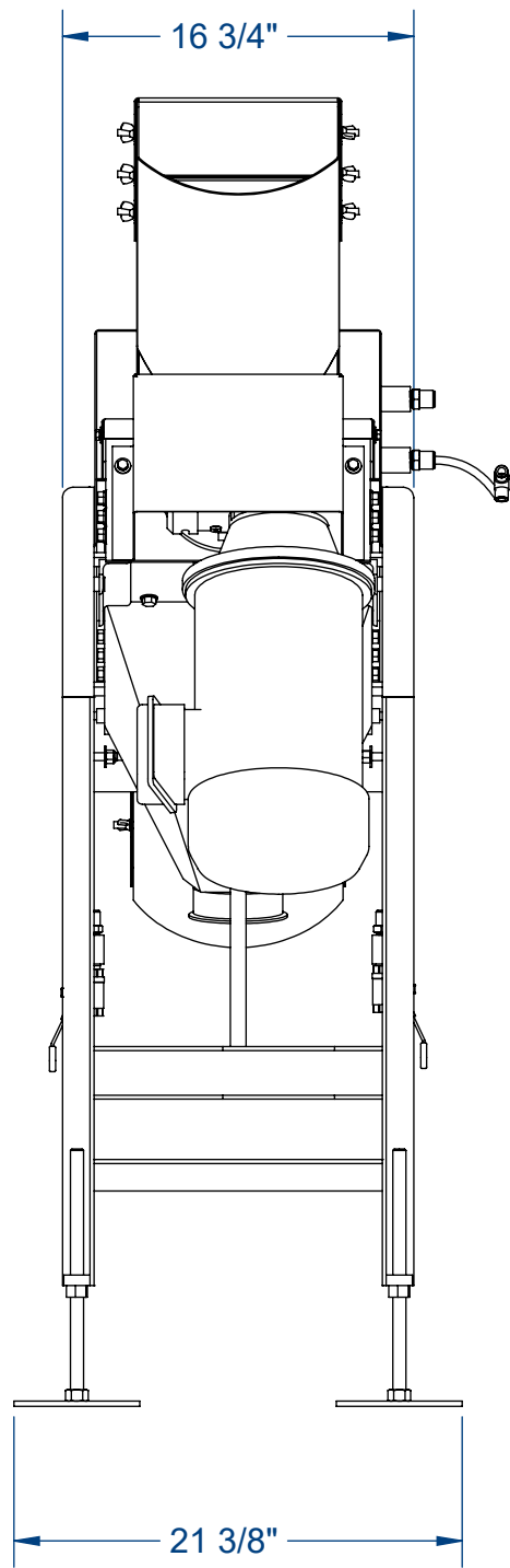
INLET VIEW
